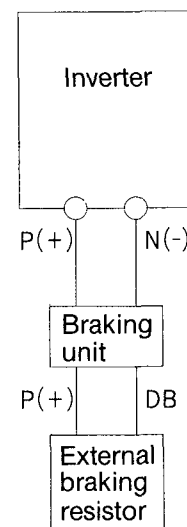
Fig. 6-1-3 Connection diagram
