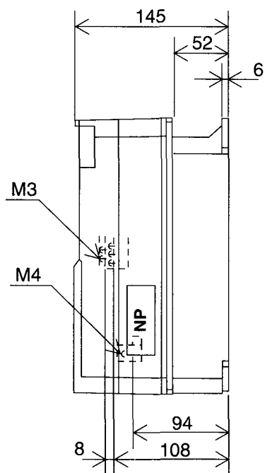
FRN1.5~3.7G9S-2 FRN0.75~3.7G9S-4
