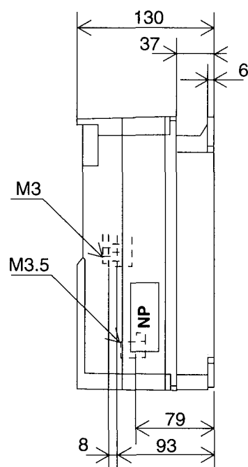
FRN0.75G9S-2 FRN0.4G9S-4
