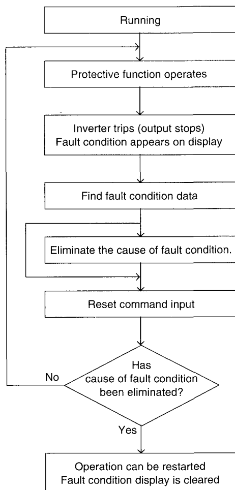
Fig. 11-1-1 Protective function operation and resetting
