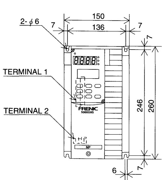
FRN1.5~3.7G9S-2 FRN0.75~3.7G9S-4
