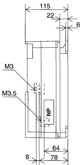
FRN0.2~0.4G9S-2
