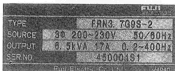
Fig. 3-2 Name plate
