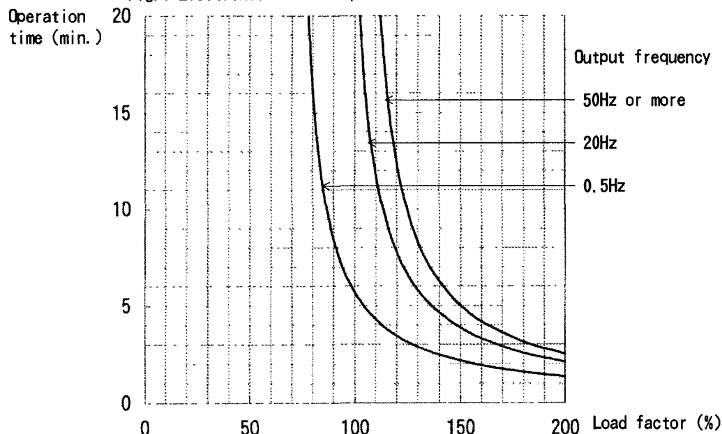
Fig.1 Electronic overload protection characteristic
