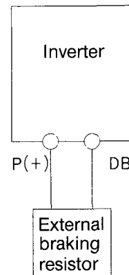
Fig. 6-1-2 Connection diagram
